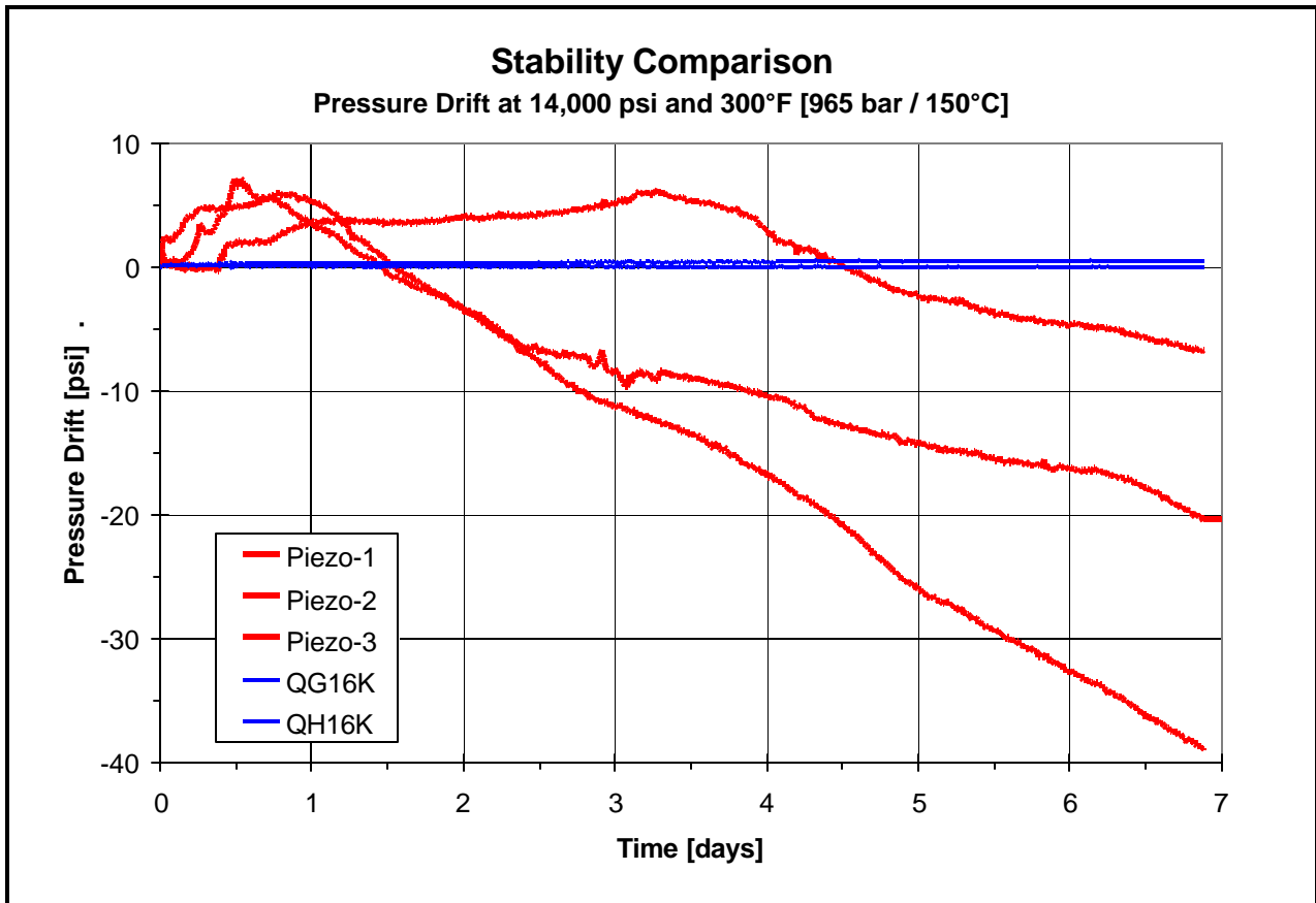
Figure 4: Drift Comparison Between Quartzdyne 16K and Piezoresistive Sensors
